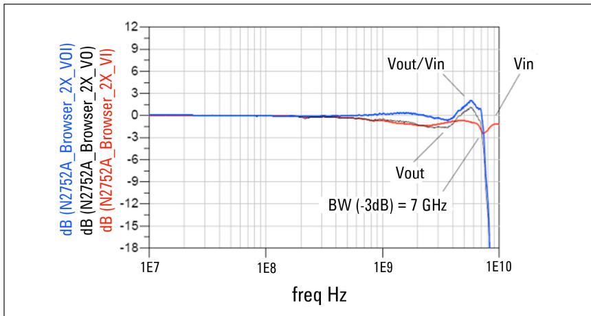
Figure 6. Vout/Vin frequency response of N2752A (at 2:1) with browser tip
